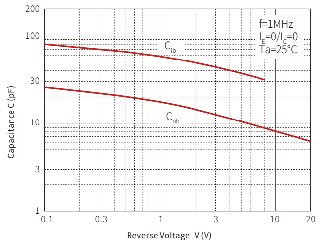
C_{ob}/C_{ib} \text{ — } V_{CB}/V_{EB}
