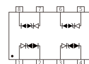
Schematic Symbol
