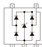
Schematic Symbol
