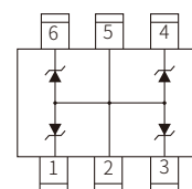
Schematic Symbol
