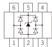
Schematic Symbol
