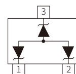
Schematic Symbol
