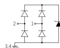
Schematic Symbol
