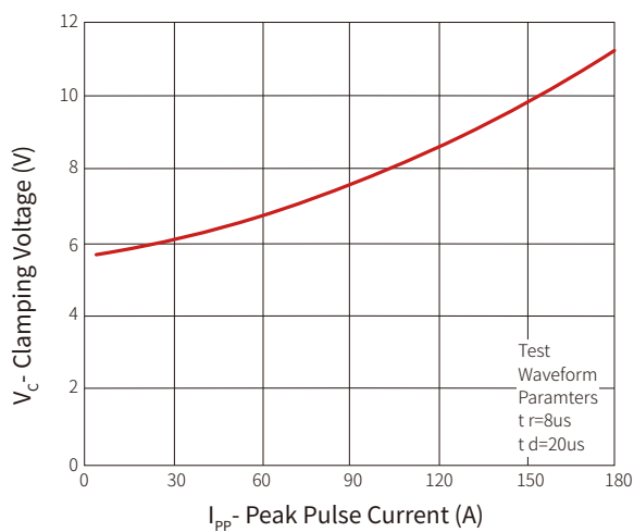
Reverse Clamping Voltage vs. Peak Pulse Current
