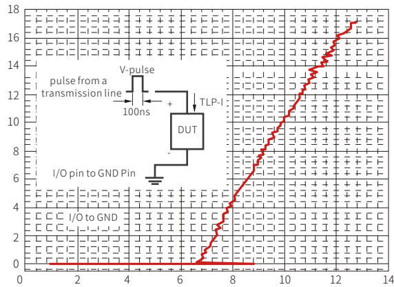
Transmission Line Pulsing (TLP) Measurement
