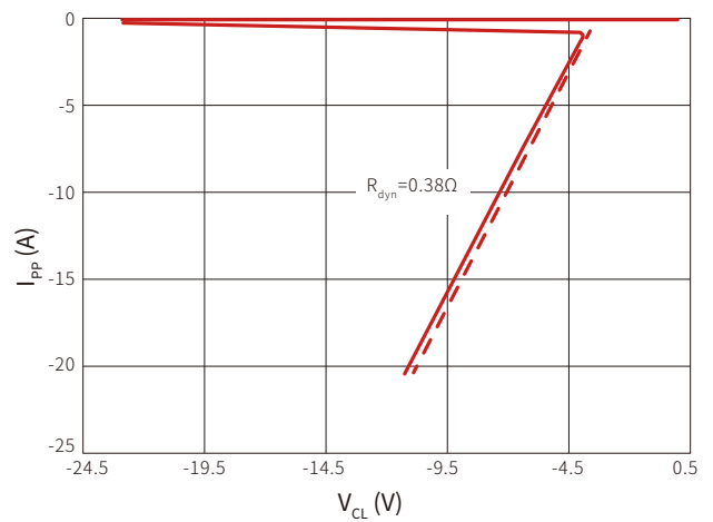
Negative Clamping voltage (TLP)
