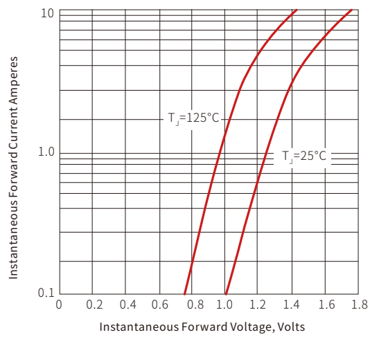
Fig. 3-Typical Forward Characteristics
