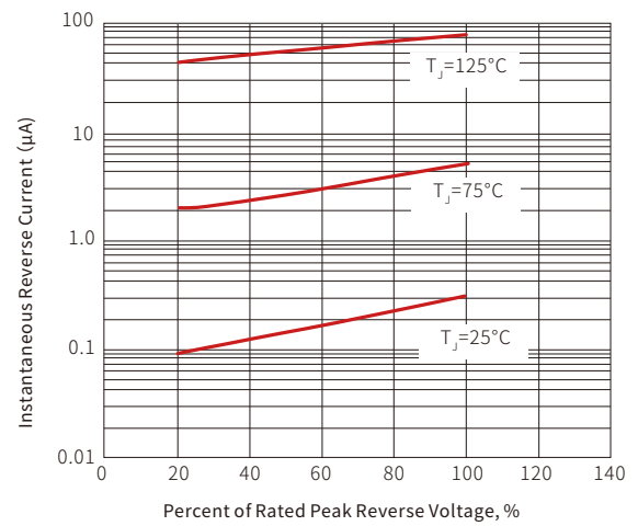
Fig. 4-Typical Revers Characteristics
