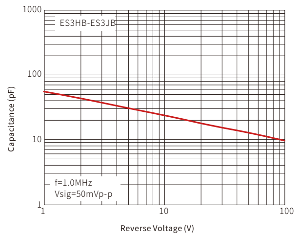
Fig. 8-Typical Junction Capacitance
