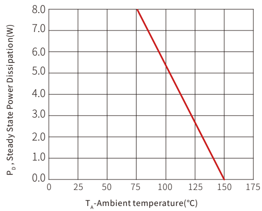
Figure 7: Steady State Power Dissipation Derating Curve
